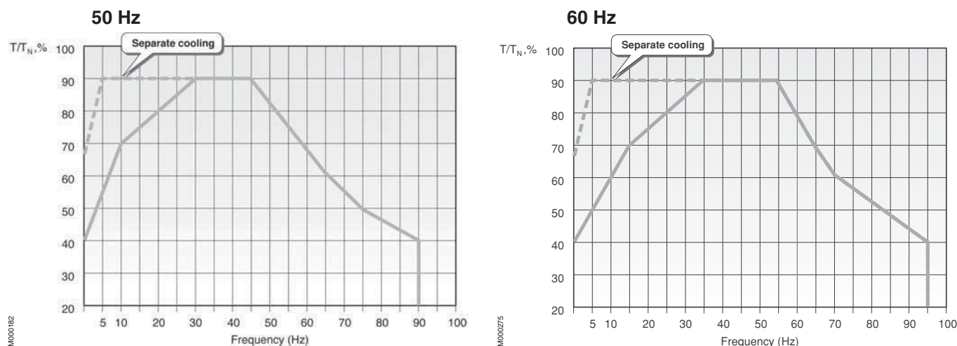
Figure 3. Non-sparking motors Ex nA, cast iron (type M3GP) and aluminum dust ignition proof motors (DIP/Ex tD T125°C), nominal frequency of motor 50/60 Hz
