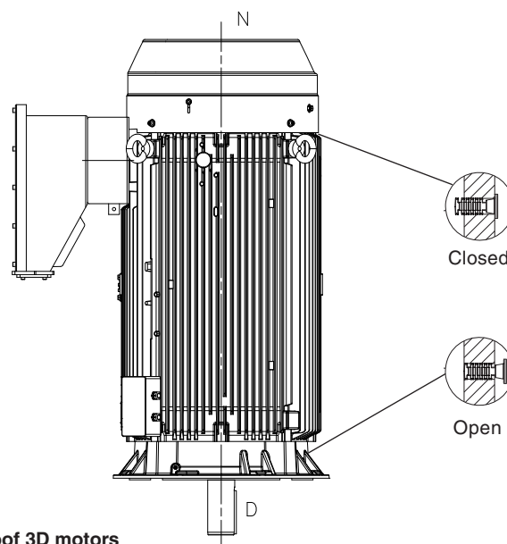
Non-sparking, dust ignition proof 3D motors As standard with drain holes and closable plugs.
