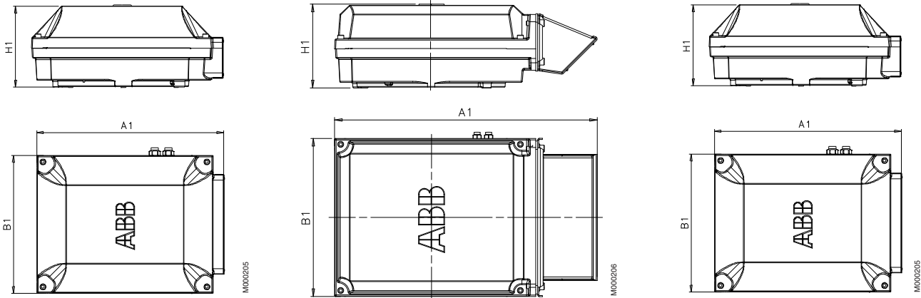
Motor sizes 280 - 315 Top- and side-mounted Terminal boxes 210, 370 Motor sizes 355 - 450 Top-mounted Terminal box 750 + adapter Side-mounted Terminal box 750
